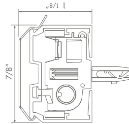
HEADRAIL SECTION
